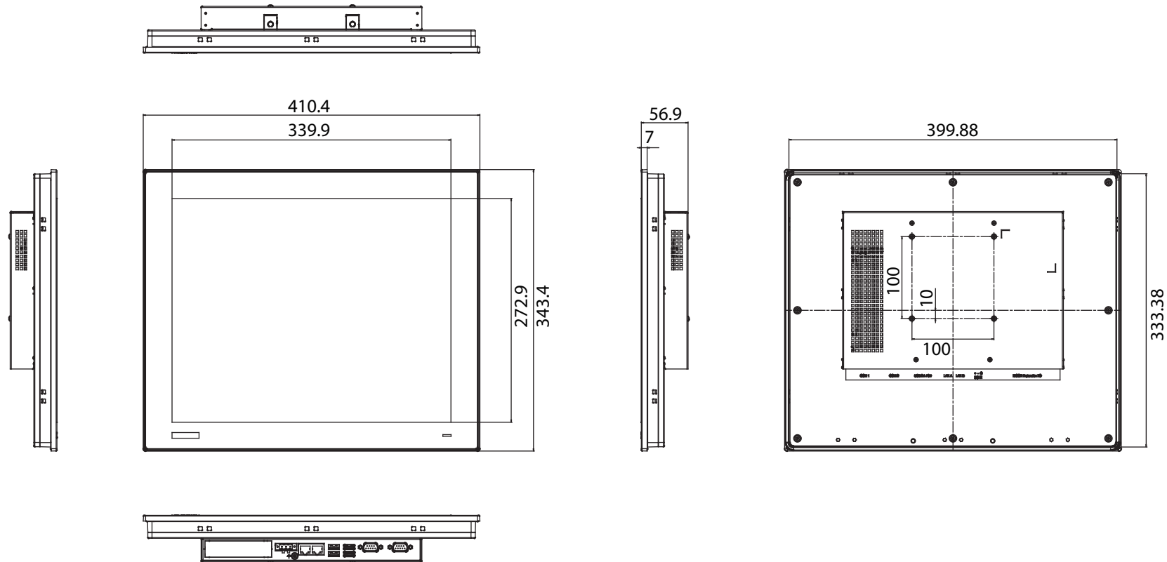
Panel Cutout Dimensions: 401.3 x 334.8 mm (15.80" x 13.18")
